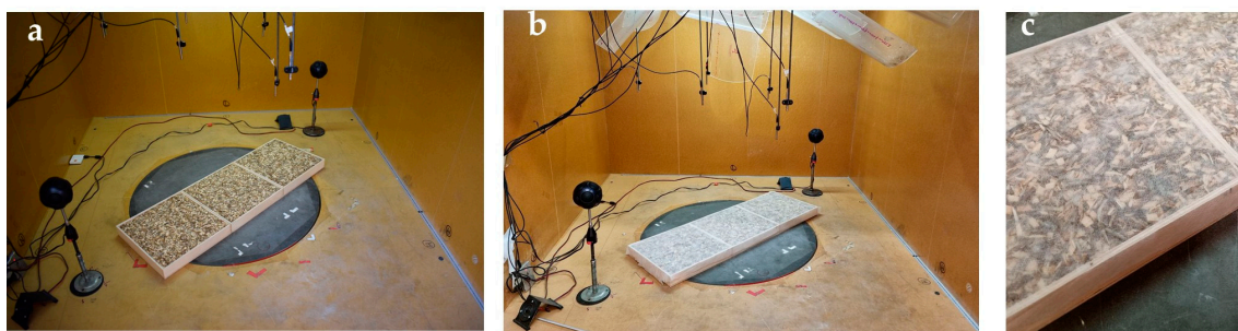
Figure 7. (a) O100|_{full} configuration; (b) O100|_{full} configuration with TNT; (c) details of the TNT.
