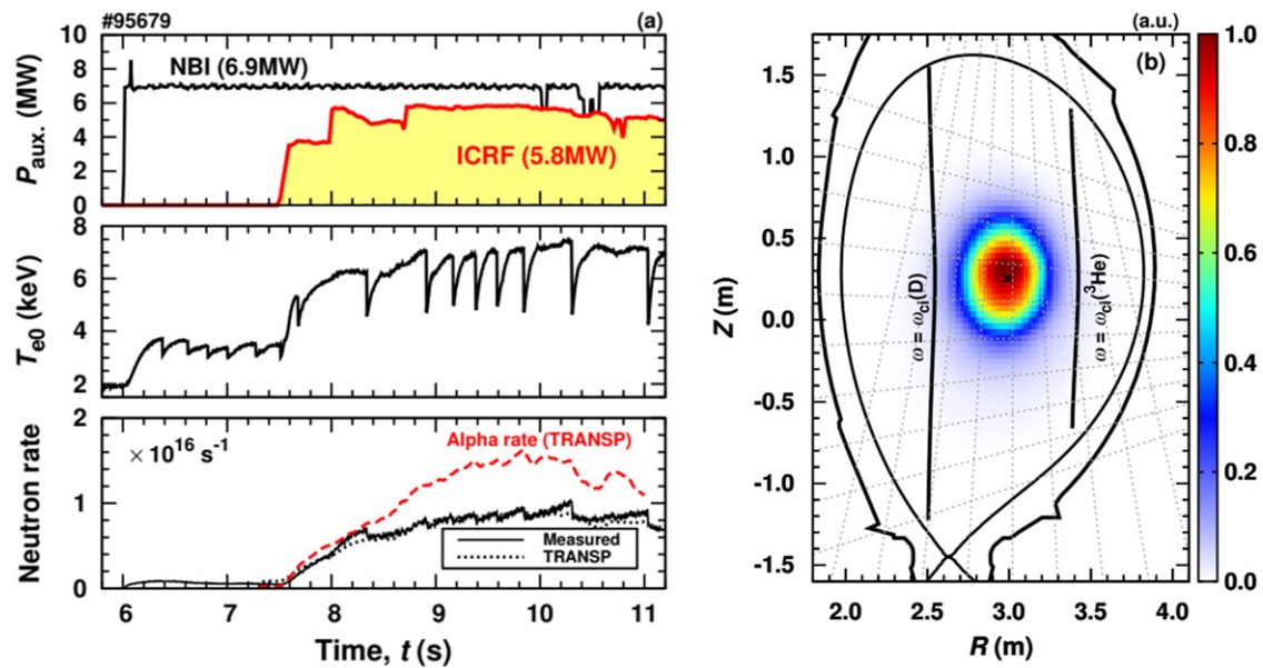
Figure 3. (a) Pulse #95679, with the three-ion D–( D_{NBI} )– ^3He scenario applied for heating and FI generation. The bottom panel shows the simulated (TRANSP) D–D neutron and D– ^3He \alpha rates. (b) Spatial profile of D–D neutron emission. Figure reproduced from [29].
