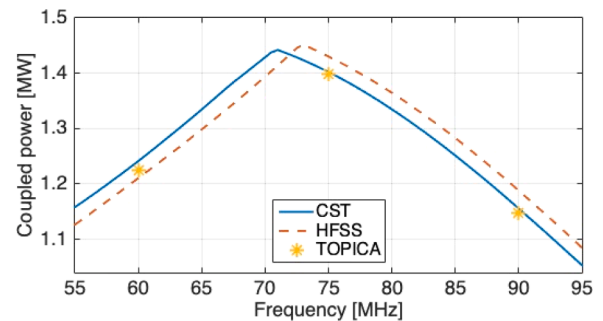
Fig. 3. Benchmark of HFSS and CST simulations with homogeneous dielectric against TOPICA results for a three-strap antenna in front of a DTT reference plasma.
