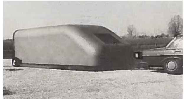
Figure 13. Trailer used to determine the rolling resistance of a vehicle [11]
