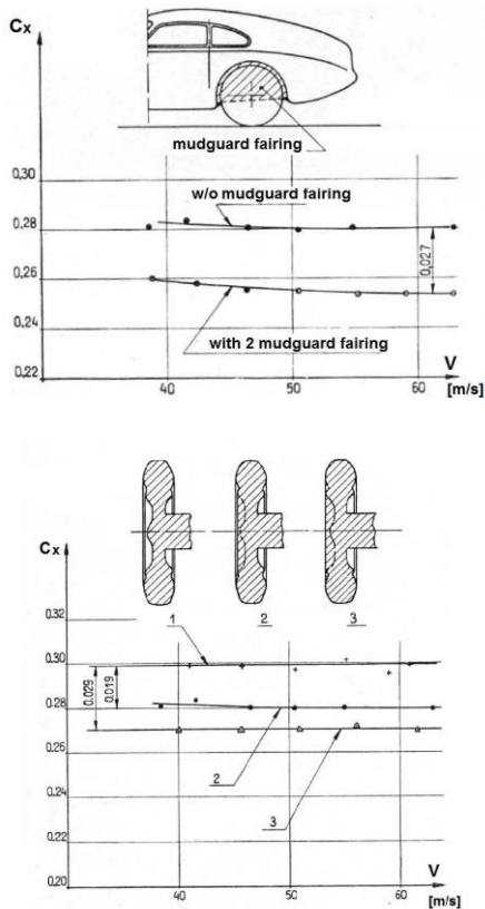
Figure 26. Significant wheel C_x reductions obtained by covering the wheel that extends from the mudguard (above) and by the profiling of the wheel disc (below) [20]
