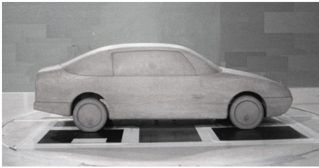
Figure 29. The Notch-back Fiat “Tito 3” car [22,23]
