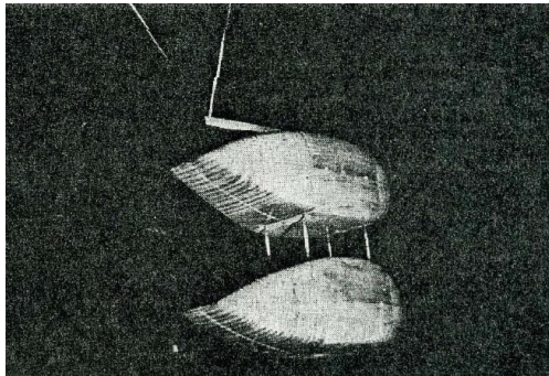
Figure 2. Basic body tested in 1:5 at a scale in the wind tunnel. The image method was used on a scaled-down model in order to simulate the effect of the ground [2]
