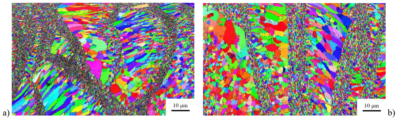
Figure 6. EBSD images of Scalmaalloy® a) before and b) after aging heat treatment.
