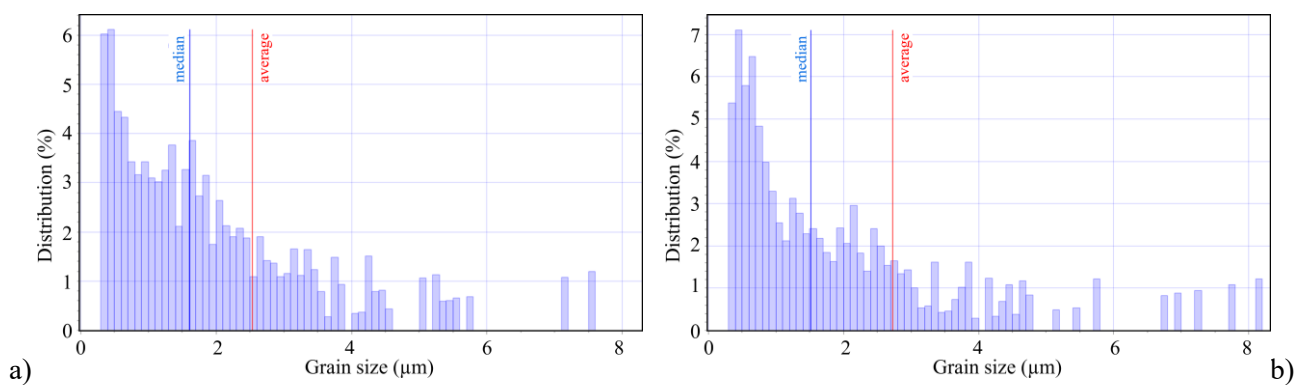
Figure 7. Grain size distribution (measured according to ASTM E2627 [28]) of Scalmaalloy® a) before and b) after the aging heat treatment.
