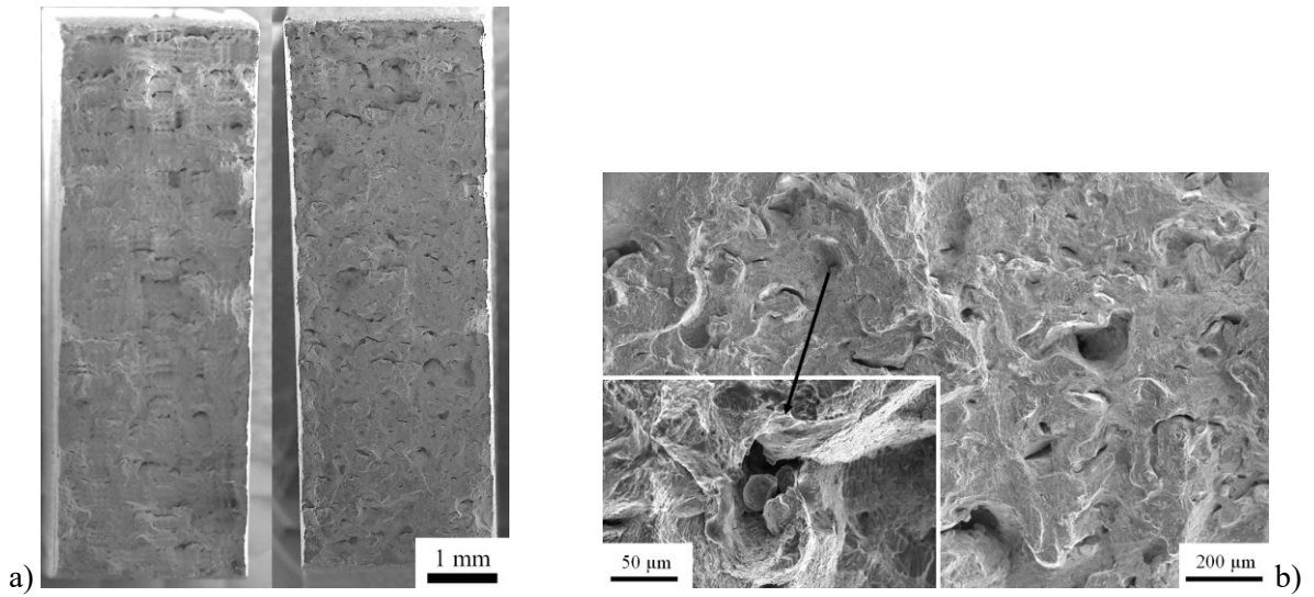
Figure 15. SEM image of the fracture surface obtained from a) the heat-treated Scalmaalloy® (“A” plate) and b) its magnification.
