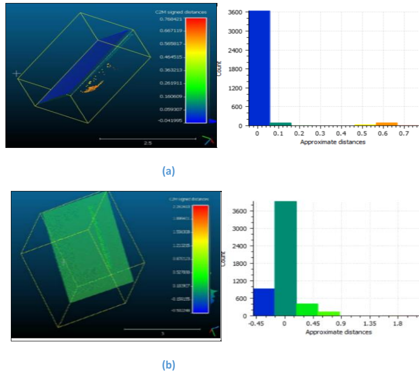
Figure 8: Overlaid TLS generated surfaces for a) flat area b) curved area
