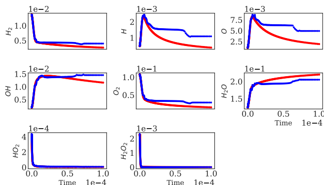
Figure 18: Comparison between the lifted with Latent Harmonics trajectory computed with the data-driven integration scheme Back and Forth (blue trajectory) and the trajectory computed from the full, unreduced equations of the kinetics (red trajectory).
