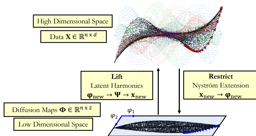
Figure 1: An illustration of our computational tools (Diffusion Maps, Latent Harmonics and Nyström Extension) for building reduced dynamical models.
