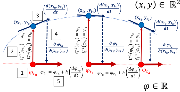
Figure 3: 1. Start integration at t = 0 from an initial condition in the reduced space \phi_{t_0} . 2. Use Algorithm 2 to compute the corresponding values of the high dimensional space variables, x_{t_0}, y_{t_0} . 3. From x_{t_0}, y_{t_0} by using the expressions of the dynamics in the high dimensional space compute the derivatives \frac{d(x_{t_0}, y_{t_0})}{dt} . 4. To obtain the reduced dynamics \frac{d\phi_{t_0}}{dt} the calculation of the chain rule is needed \frac{d\phi_{t_0}}{dt} = \frac{\partial \phi_{t_0}}{\partial x_{t_0}} \cdot \frac{dx_{t_0}}{dt} + \frac{\partial \phi_{t_0}}{\partial y_{t_0}} \cdot \frac{dy_{t_0}}{dt} , where the terms \frac{\partial \phi_{t_0}}{\partial (x_{t_0}, y_{t_0})} are computed by differentiation of the Nyström Extension formula. With known the value of \frac{d\phi_{t_0}}{dt} the value of \phi_{t_1} is estimated. By repeating the steps 2-5 integration in the Diffusion Maps coordinates is achieved.
