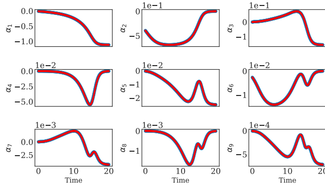
Figure 16: Comparison between the lifted with Latent Harmonics trajectory computed with the data driven integration scheme Back and Forth (blue trajectory) and the trajectory coming from the spectral odes (red trajectory).
