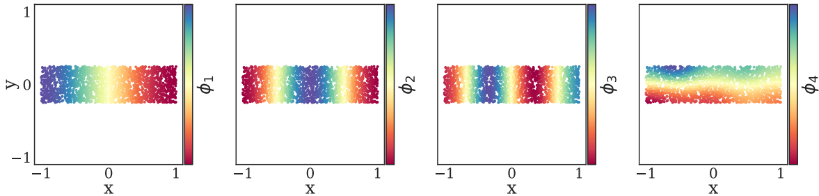
Figure 14: The first four (non-trivial) Diffusion Maps coordinates are colored as function on the data set.
