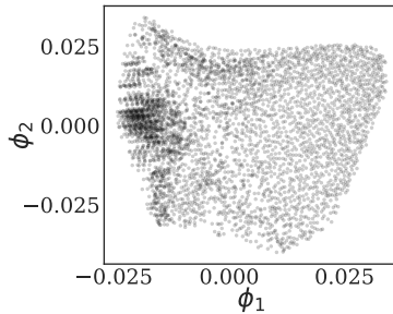
Figure 8: The two dimensional manifold in terms of the independent eigenvectors \phi_1 and \phi_2 discovered on Chemical Kinetics example.
