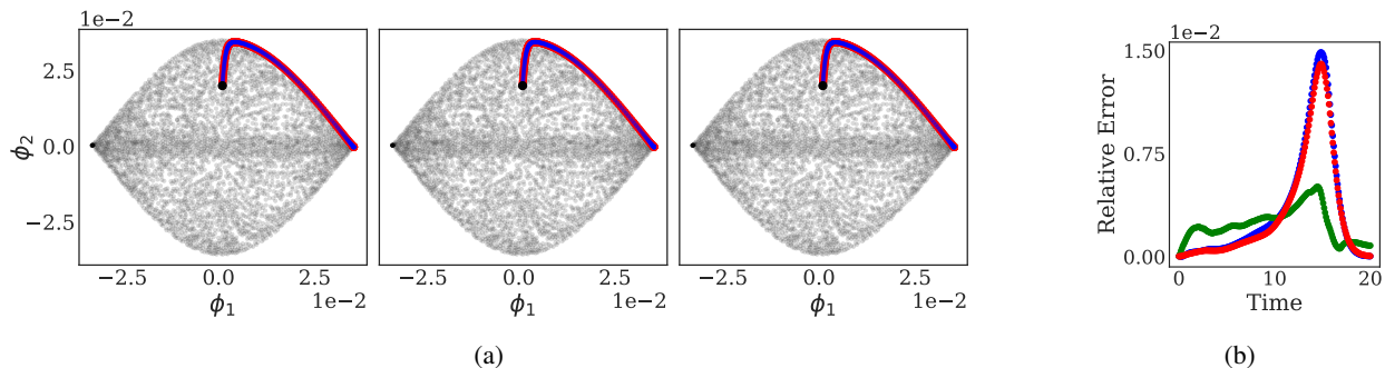
Figure 5: (a) A comparison between a trajectory computed with the three data-driven frameworks TaLHI, BF, and GT, respectively is shown (blue color) against with a restricted (with Nyström Extension) trajectory obtained from the spectral ODEs (red color) for the Chafee-Infante example. (b) The relative error between the data-driven trajectories and the reduced trajectory from the unreduced equations.
