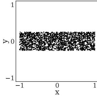
Figure 13: Data points collected from rectangle with sides' ratio 4:1.
