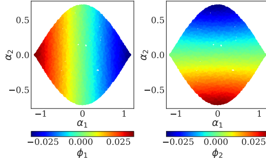
Figure 4: The first two Fourier modes \alpha_1 and \alpha_2 are colored with the two independent Diffusion Maps coordinates \phi_1 (left) and \phi_2 (right). The Fourier mode \alpha_1 is one-to-one with \phi_1 and \alpha_2 is one-to-one with \phi_2 .
