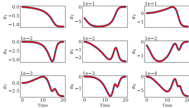
Figure 17: Comparison between the lifted with Latent Harmonics trajectory computed with the data-driven integration scheme Grid Tabulation (blue trajectory) and the trajectory coming from the spectral odes (red trajectory)
