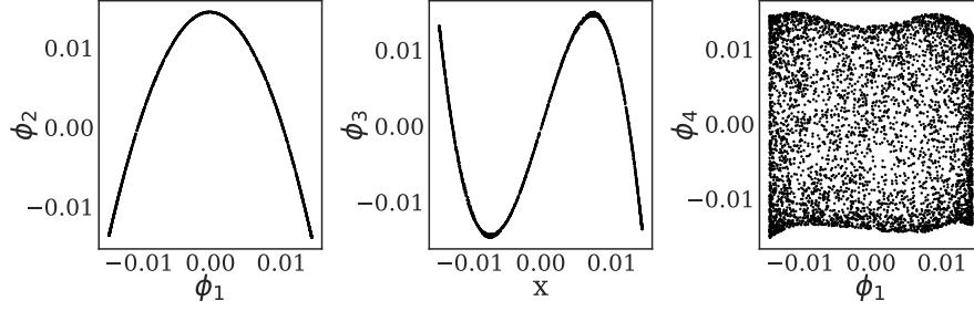
Figure 15: The first non-trivial coordinate \phi_1 is plotted as against the eigenvectors \phi_2, \phi_3, \phi_4 respectively, .
