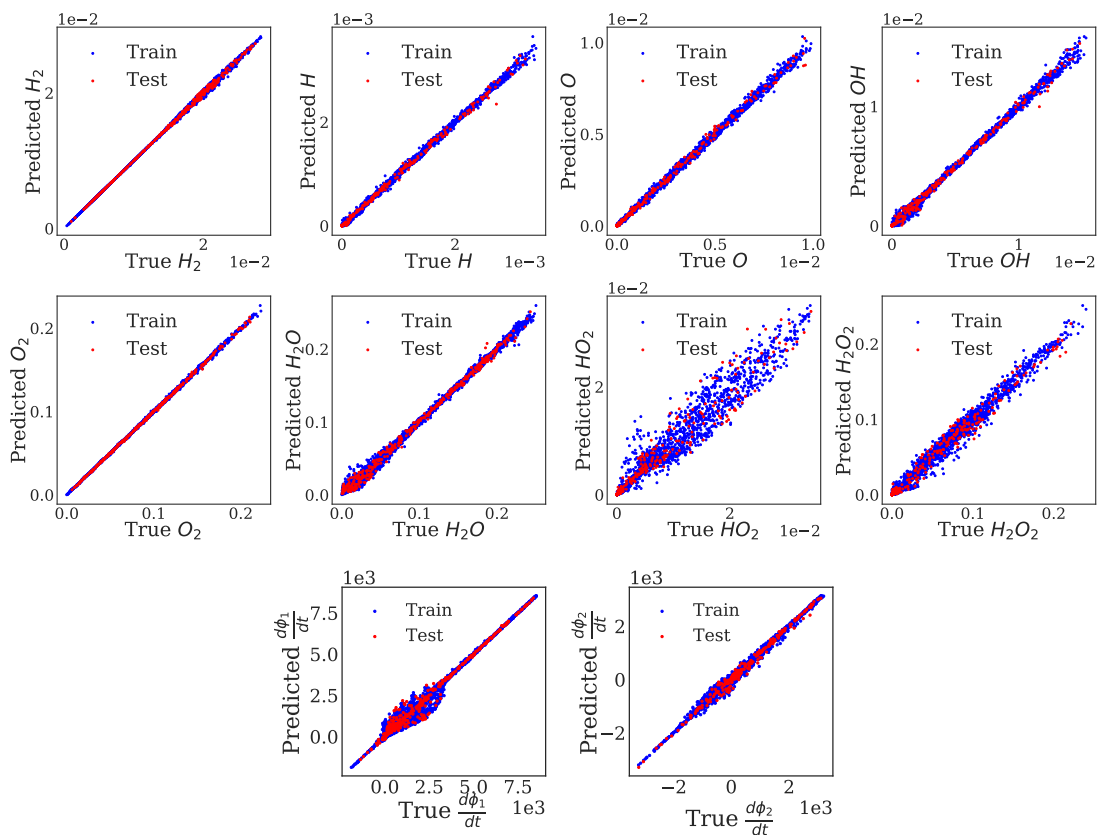
Figure 21: The true values of functions of interest plotted against the predicted with Latent Harmonics for the Kinetics example. Blue color points represent the training points and red points the test.
