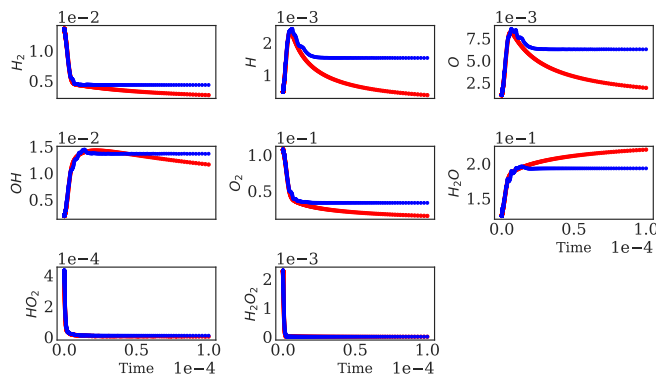
Figure 19: Comparison between the lifted with Latent Harmonics trajectory computed with the data-driven integration scheme Grid Tabulation (blue trajectory) and the trajectory computed from the full, unreduced equations of the mechanism (red trajectory). The reduced trajectory due to numerical errors is not able to continue since it leaves the manifold.
