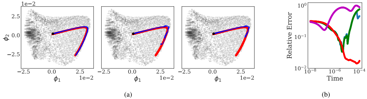
Figure 9: (a) A comparison between a trajectory computed from the three data-driven frameworks TaLHI, BF, and GT, respectively is shown (blue color) and a restricted (with Nyström Extension) trajectory obtained from the spectral ODEs (red color) for the example from Chemical Kinetics. (b) The relative error in time of the four data driven approaches for each point along the simulated trajectory, BF (blue), GT (green), TaLHI (red), Chiavazzo et al [6] (magenta), each compared to the restricted with Nyström Extension trajectory of the full dynamics.
