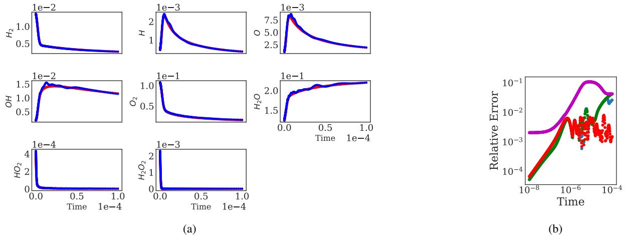
Figure 10: (a) Comparison between the lifted with Latent Harmonics trajectory computed with the data-driven integration scheme Back and Forth (blue trajectory) and the trajectory computed from the full, unreduced equations of the kinetics (red trajectory). (b) The relative error in the ambient space between the lifted data driven schemes and a trajectory of the full dynamics, BF (blue), GT (green), TaLHI (red), Chiavazzo et al [6] (magenta). The lifting in our proposed data-driven schemes was performed with Algorithm 2 and the one in Chiavazzo et al. with local Geometric Harmonics.
