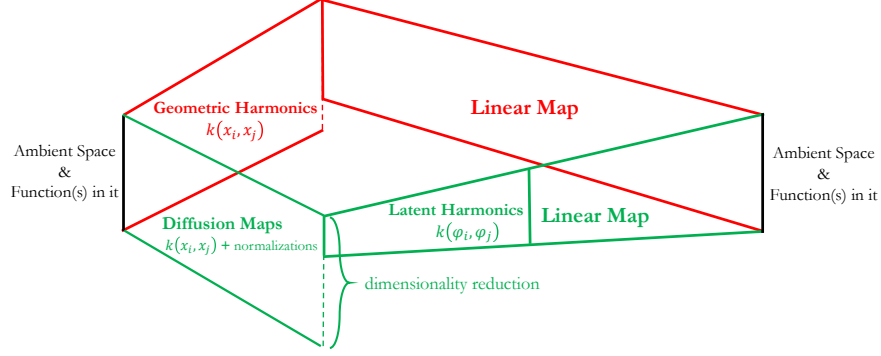
Figure 2: The upper, red schematic shows the mapping constructed from the ambient space and functions in it, via Geometric Harmonics, back to the ambient space and functions in it. The lower, green schematic illustrates our proposed approach that involves (a) first computing Diffusion Maps to discover the intrinsic geometry of a given data set (that might also lead to dimensionality reduction) and then (b) mapping from the reduced obtained latent space back to the ambient space and functions in it.
