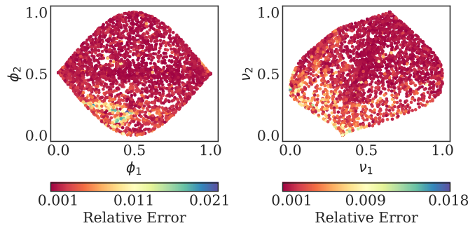
Figure 11: The relative error \frac{|\phi_i - \hat{\phi}_i|}{\phi_i} of the forward mapping, f : N \rightarrow \Phi is shown on the left as a function on the original values of the Diffusion Maps coordinates. The relative error \frac{|\nu_i - \hat{\nu}_i|}{\nu_i} of the backward mapping f^{-1} : \Phi \rightarrow N is shown on the right. In both cases the coordinates are rescaled in the range 0 to 1.
