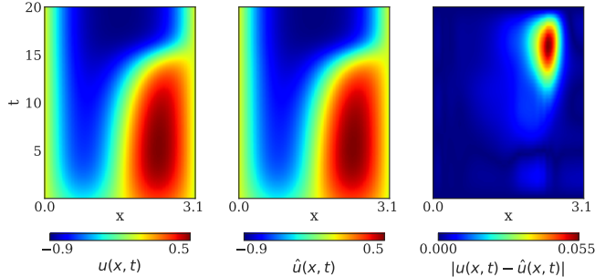
Figure 7: A trajectory u(x, t) of the Chafee Infante PDE, Equation (3), integrated with Finite Differences (left) compared to a lifted & reconstructed trajectory \hat{u}(x, t) obtained with the data-driven scheme TaLHI. The absolute error of u(x, t) and the data-driven trajectory \hat{u}(x, t) is shown in the right.
