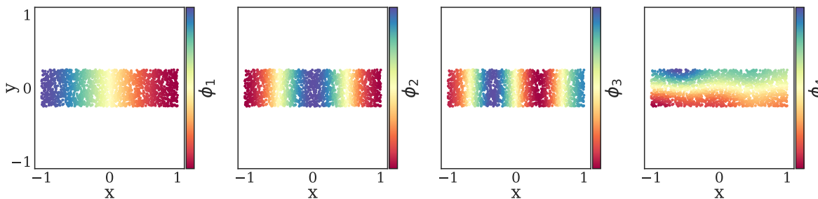
Figure 14: The first four (non-trivial) Diffusion Maps coordinates are colored as function on the data set.
