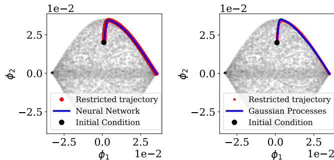
Figure 12: data-driven Integration with a Neural Network (on the left) and Gaussian Processes (on the right).
