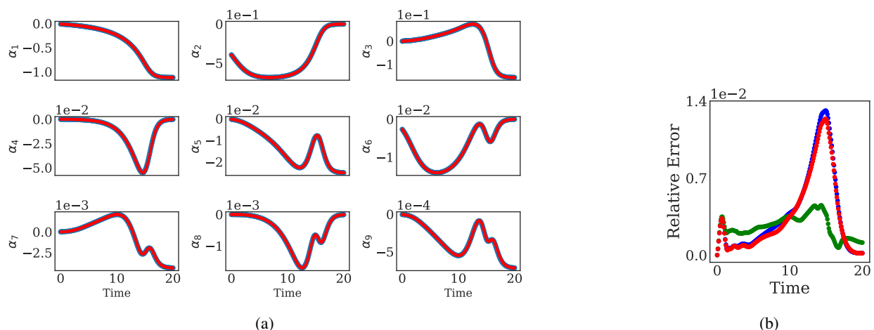
Figure 6: (a) A comparison between the lifted with Latent Harmonics trajectory computed from the data-driven integration scheme TaLHI (blue color) and the trajectory computed from the full, unreduced equations (red color) is shown for the first nine Fourier Modes. (b) The relative errors in time between the data-driven trajectories and the trajectory from the full, unreduced equations, BF (blue), GT (green), TaLHI (red).
