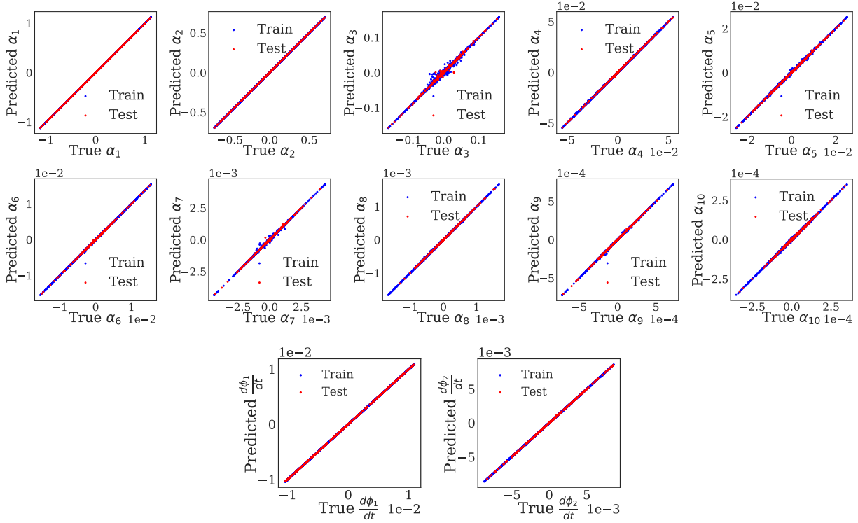
Figure 20: The true values of functions of interest plotted against the predicted with Latent Harmonics for the Chafee-Infante PDE. Blue color points represent the training points and red points the test.
