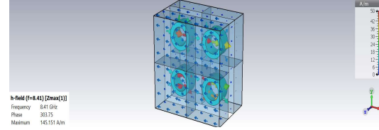
Fig. 8. Surface currents at 8.41 GHz.
