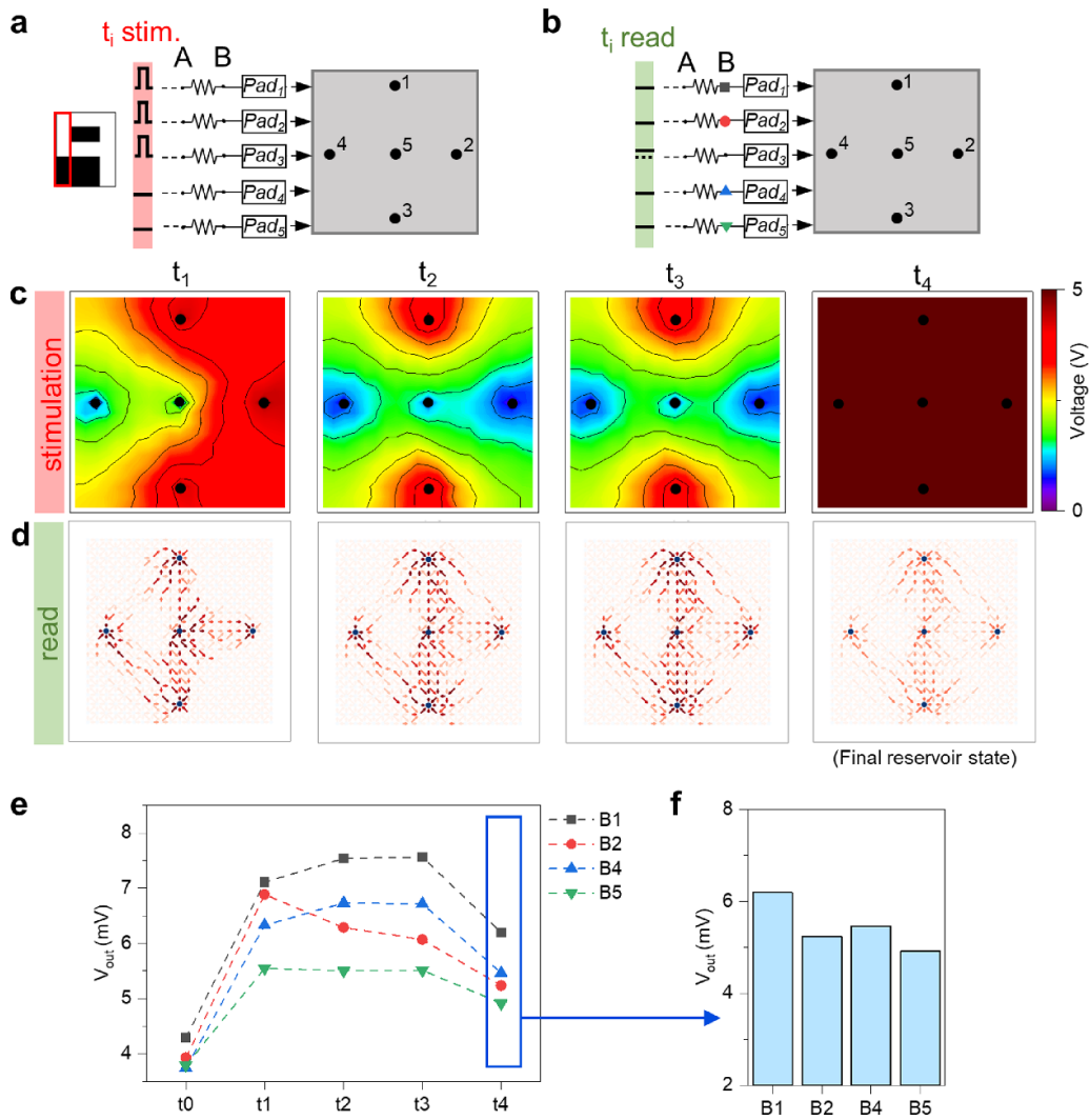
Figure 6. Evolution of internal NW network reservoir dynamics in RC configuration c, during stimulation with digit ‘9’. Configuration during (a) stimulation and (b) read sections. In this case, the stimulation configuration in panel (a) (here schematized as in the first timeframe of stimulation with digit ‘9’) has not to be changed over timeframes since no channels has to be selected and no floating electrodes are present. (c) Voltage distribution over the NW network during the stimulation section of each timeframe and (d) conductance maps evaluated during the read section of each timeframe obtained with the grid-graph model. In panel (c) black lines represent equipotential lines while in panel (d) the red intensity of edges is proportional to the edge conductance while the edge arrow indicates the current flow direction. (e) Evolution of reservoir output voltages over timeframes and (f) corresponding histogram of final reservoir state. The final reservoir state corresponds to the reservoir state to be passed to the readout for classification. Output voltages in panels (e) and (f) were evaluated during the read section of each timeframe, by exploiting the configuration reported in panel (b). In particular, the different symbols used to represent output voltages in panels (e) correspond to symbols exploited to highlight the different B terminals in panel b, where output voltages are recorded.
