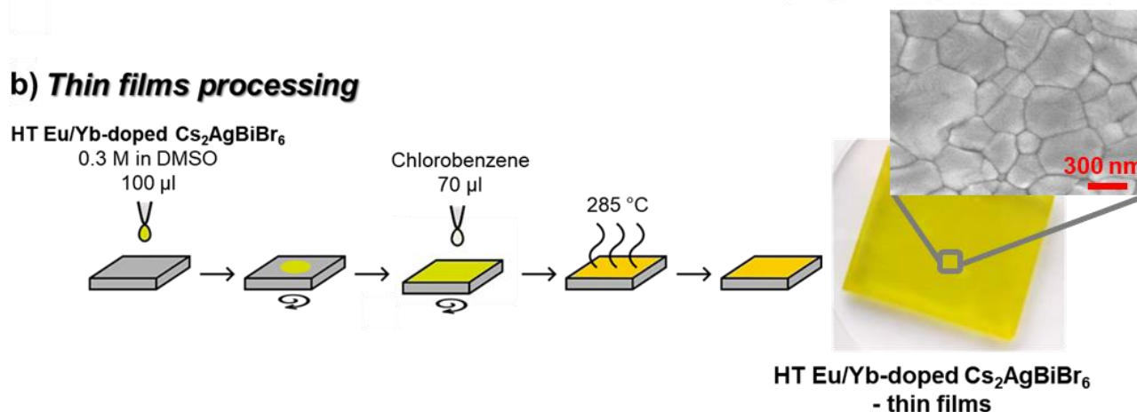
Figure 1. Synthesis, characterization and thin film processing of bulk Eu- and Yb-doped \text{Cs}_2\text{AgBiBr}_6 . a) Sketch of the hydrothermal synthesis process, with picture and SEM image of a prototypical crystalline product. b) Sketch of the anti-solvent method used for the preparation of thin films, with picture and top-view SEM image of a prototypical film.
