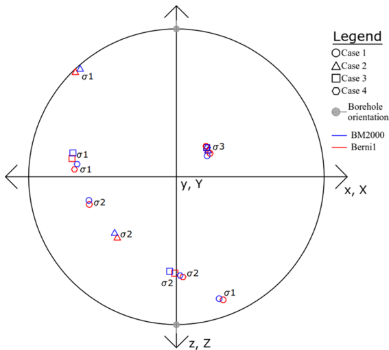
Fig. 5 Stereogram of the maximum principal stresses calculated with BerniI and BM2000 software to validate the transverse isotropic case. The symbols \circ , \Delta , \square , \hexagon , respectively, identify the maximum principal stresses calculated \sigma_1 , \sigma_2 , \sigma_3 , in MPa, for the 4 cases analysed
