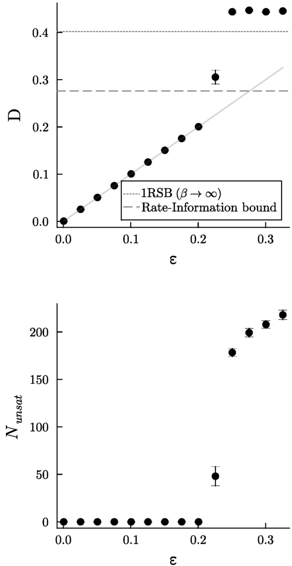
FIG. 13. Performance of max-sum with reinforcement on source vectors made by perturbing the all-zeros codeword with \epsilon n bit flips. n = 1800 , \Lambda = \{\lambda_2 = 0.45, \lambda_3 = 0.55\} , P = \{p_3 = 1\} , R = 0.15 , average over 50 instances. The upper panel shows the average distortion, with the Shannon bound and 1RSB prediction for a symmetric source as references. The lower panel shows the number of unsatisfied factors.
