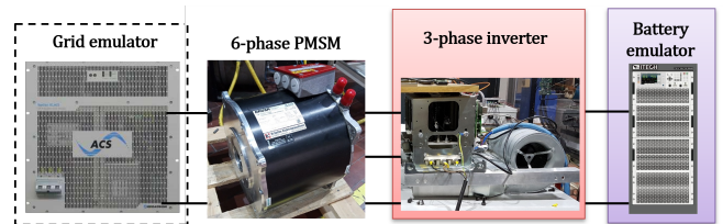
FIGURE 14. Test bench for experimental validation of IFI-OBC.
