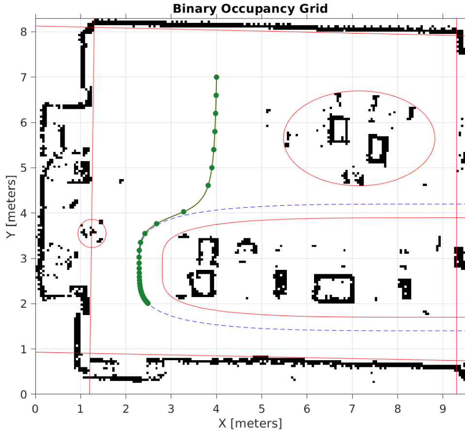
Fig. 2.8 MATLAB simulation plot for the SGP algorithm. A subset of the computed waypoints is highlighted with green dots.
