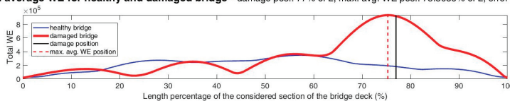
Filtered average WE for healthy and damaged bridge - damage pos.: 77% of L, max. avg. WE pos.: 75.3086% of L, error = -2.1966%
