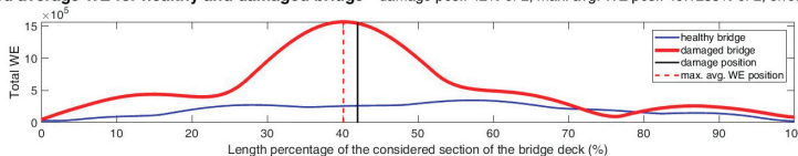
Filtered average WE for healthy and damaged bridge - damage pos.: 42% of L, max. avg. WE pos.: 40.1235% of L, error = -4.468%
