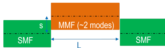
Figure 1: Schematic representation of the interferometric sensor SMS in which an FBG has been inscribed in the multimode section. SMF: standard single mode fiber; MMF: multimode fiber that supports the propagation of two modes that in this case is an enhanced backscattering fiber (EBF).
