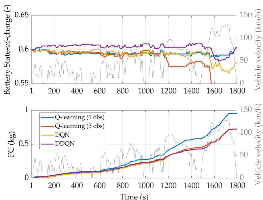
Figure 8. Battery SOC (upper chart) and FC (lower chart) profiles obtained by the RL agents on the WLTC in the case of FC-oriented reward.
