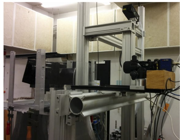
FIG. 2. Planar-PIV setup.
