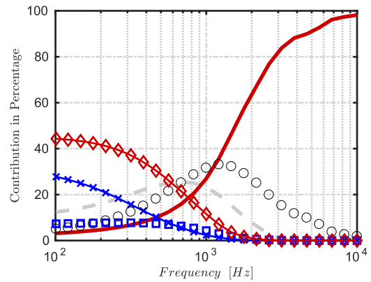
FIG. 25. Regional contribution of the MS term at RMP 26. Legends: red solid curve—inner layer; black open circles—inner-middle layer; blue open squares—inner-outer layer; gray dashed line—middle layer; red curve with open diamonds—middle-outer layer; and blue curve with crosses—outer layer.
