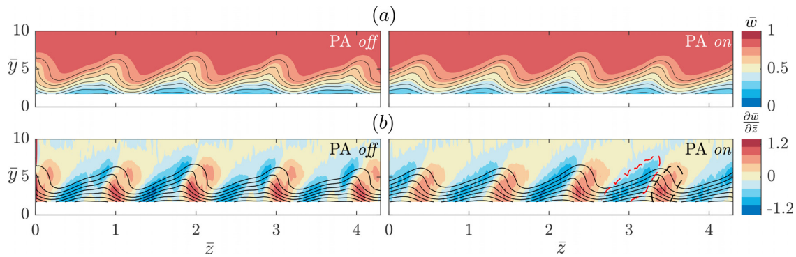
FIG. 9. (a) Time-averaged velocity fields \bar{w} and (b) spanwise gradient of mean flow \partial\bar{w}/\partial\bar{z} for the DRE- H case. Plane location is at x/c_x = 0.225 , and black iso-lines illustrate \bar{w} , ten levels from 0 to 0.9. The regions outlined by dashed lines in (b) are based on thresholds of -0.23 and 0.5 .
