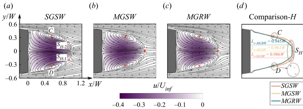
Figure 12. Comparison of averaged planar velocity magnitude u/U_{inf} contour overlaid with 2-D streamlines on the horizontal plane z/W=0.51 . (a) SGSW , (b) MGSW , (c) MGRW . The red triangles (vortex centre), red square and circle (saddle point). The red upper triangle (upper vortex centre), red lower triangle (lower vortex centre), red square (saddle point). (d) Comparison of the positions of the vortex centre and saddle point, and horizontal planar recirculation region. SGSW (orange colour), MGSW (yellow colour), MGRW (cyan colour). Flow is from left to right in these images. SGSW (orange solid line).
