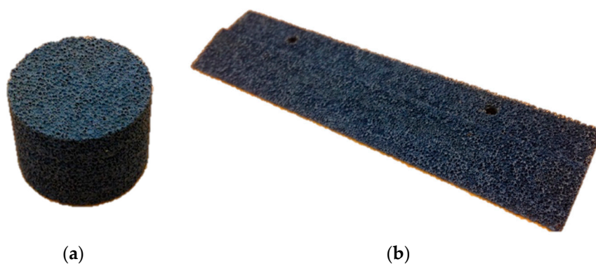
Figure 1. Examples of (a) cylinder of 2 cm diameter, and (b) trailing edge insert of 14 cm length manufactured by water-cutting of 1200 \mu\text{m} permeable foam.
