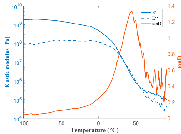
Figure 5. DMA measurements for solvent-based paint system.
