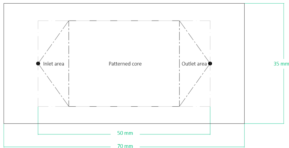
Figure 3. Layout of the microfluidic device, showing the inlet and outlet area and the pattern. The linear dimensions refer to the total extension of the devices and the inlet–outlet port distance.
