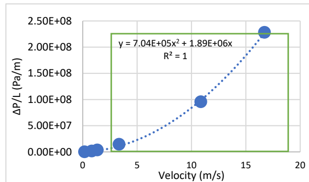
Fig. 3. Hydraulic characteristic (pressure gradient as a function of the average fluid velocity in the MCs) computed for the 6 MC connected in parallel (solid symbols), and quadratic fit according to Eq [1]. (marked area represents the turbulent fluid regime).
