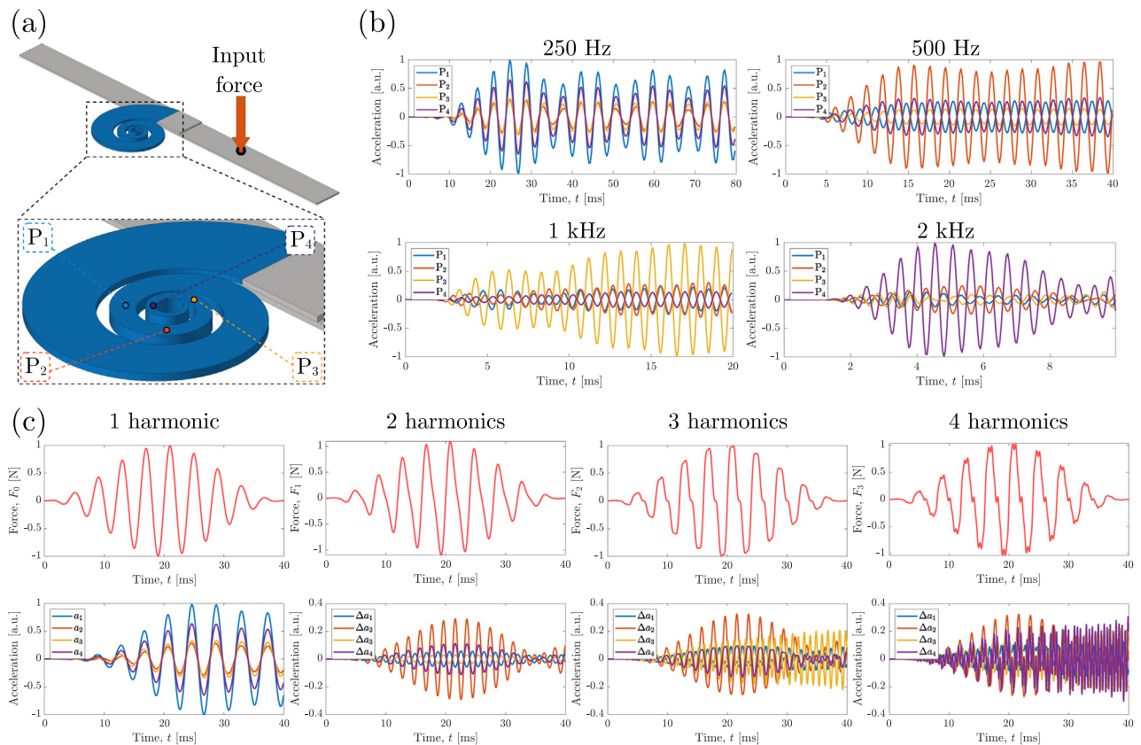
Fig. 5. Sensing application for the cochlea-inspired resonator as a frequency detection device of waves traveling in a beam. (a) An input force is applied at the upper face of the beam, with output points on the cochlea labelled as P_1 , P_2 , P_3 , and P_4 , with increasing \theta coordinates. (b) Computed out-of-plane accelerations, normalized with respect to the largest acceleration value for each input frequency: 250 Hz, 500 Hz, 1 kHz, and 2 kHz. Maximum corresponding amplitudes are detected at P_1 , P_2 , P_3 , and P_4 , respectively. (c) Input force (first row) and normalized acceleration outputs (second row) considering input signals with increasing number of harmonics, namely 1 harmonic (250 Hz), 2 harmonics (250 and 500 Hz), 3 harmonics (0.25, 0.5, and 1 kHz), and 4 harmonics (0.25, 0.5, 1, and 2 kHz).
