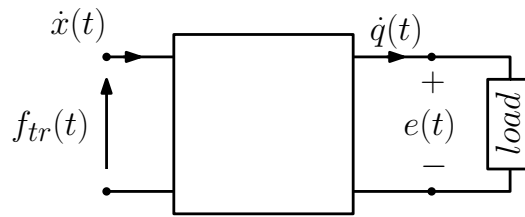
Figure 3. Piezoelectric transducer as an electromechanical two-port closed on an electrical load. At the left port are mechanical quantities: velocity \dot{x} and force f_{tr}(t) . At the right port are electrical quantities: current \dot{q} and voltage e(t) .
