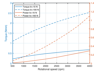
Fig. 31: Bearings 61816 theoretical friction torque and power losses with radial load kr = 10 N and kr = 100 N. Fig. 32: Bearings 6002 theoretical friction torque and power losses with radial load kr = 10 N and kr = 100 N.
