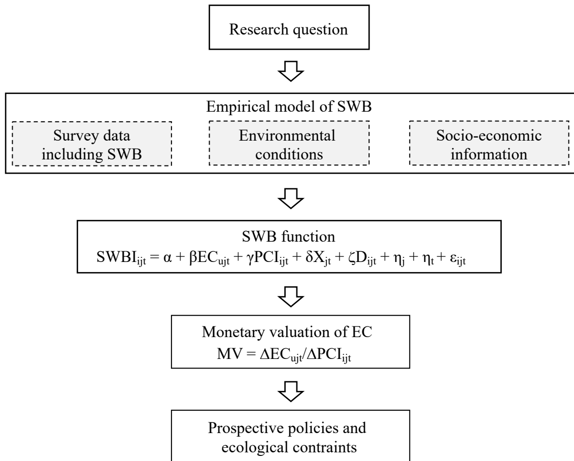
Figure 2 Research workflow
