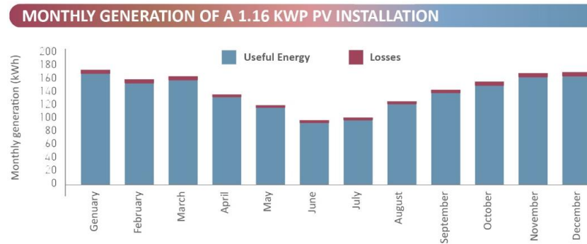
Fig. 5. Monthly simulation for a 1.16kWp PV system in Buenos Aires (1650 kWh/year ( \pm 10 )).
