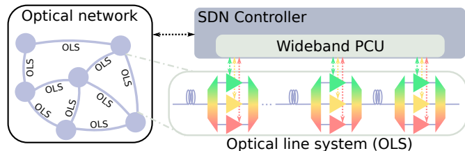
Fig. 2. Illustration of multiband PCU performing the power control for an OLS inside an optical network.
