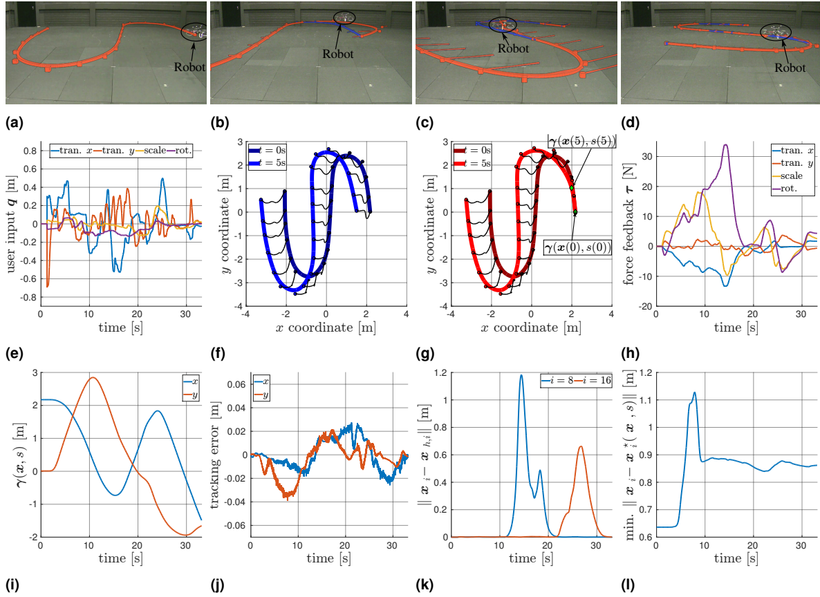
Figure 12. Experiment 1: open path. (a)-(d) Snapshots from the experiment with an overlay of the paths \gamma_S(\mathbf{x}) (red) and \gamma_S(\mathbf{x}_h) (blue). (a) Initial condition. (b) The path is being translated. (c) The path is being rotated. (d) The path is scaled down. (e) Input device's configuration q controlled by the user to give the commands. (f) Evolution of the desired path \gamma_S(\mathbf{x}_h) in the first five seconds. The circles are the control points and the black lines show their trajectories. (g) Evolution of the desired path \gamma_S(\mathbf{x}) in the first five seconds. The circles are the control points, the black lines show their trajectories and the green marker indicates the point \gamma(\mathbf{x}(t), s(t)) tracked by the robot. (h) Force feedback. (i) Reference trajectory for the robot. (j) Robot's trajectory tracking error. (k) Mismatch \|\mathbf{x}_i - \mathbf{x}_{h,i}\| for individual control points. (l) Minimum distance from the singular curves.
