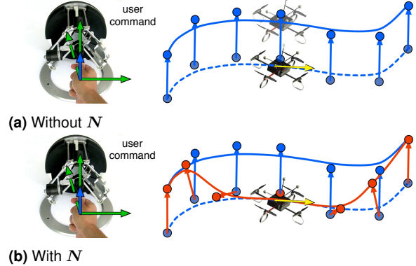
Figure 5. User commanding a translation (blue arrow) to the path \gamma_S(\mathbf{x}_h) (blue line), while the robot is traveling it with nonzero speed (yellow arrows). a) Without the blending filter, the travelled path \gamma_S(\mathbf{x}) follows exactly the command, but the resulting motion is unfeasible for the robot. b) When using the blending filter (16) and (17), the local geometric properties of \gamma_S(\mathbf{x}) are preserved and the path translation does not incorrectly affect the instantaneous motion of the robot.
