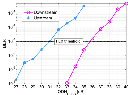
Fig. 4: Performance of the upstream and downstream transmission in terms of BER vs ODN loss.
