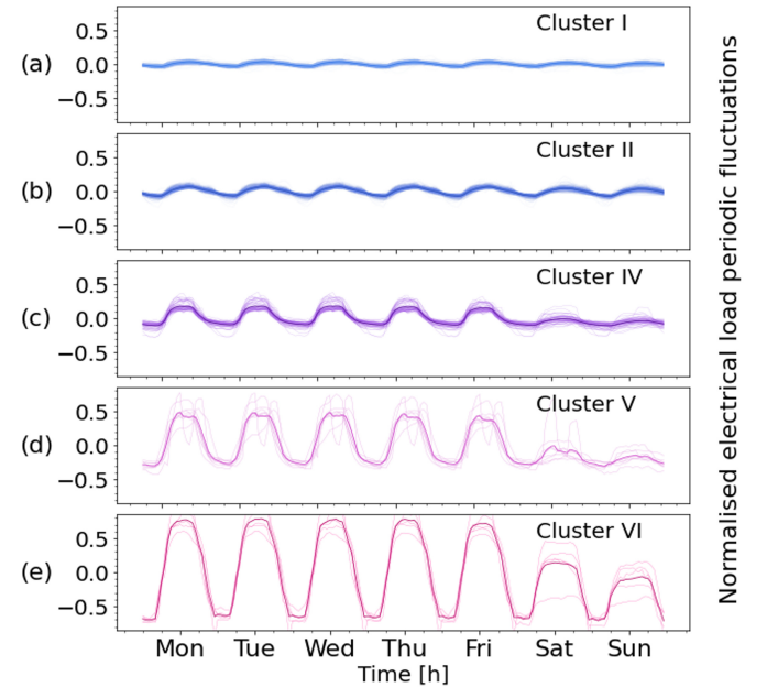
Fig. 5: Significant RPC clusters resulting from the best configuration
