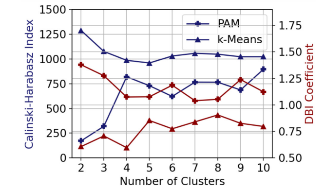
Fig. 4: CVIs comparison for the best performing algorithms, k-Means and PAM, according to different configurations
