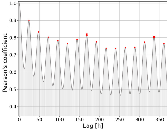
Fig. 2: Analysis of time serie auto-correlation, considering electrical measurements from a Central Office
