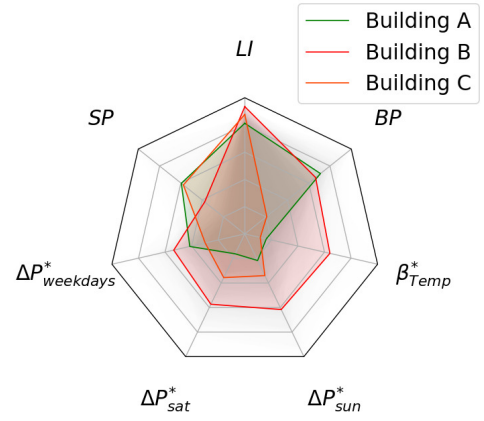
Fig. 8: Visualization of the energy KPIs characterizing efficient and bad performing TLC buildings
