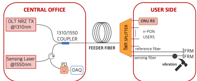
Fig. 2. PON architecture used as a Michelson interferometer, with 2 optical ports of the last PON splitter reserved for building structural monitoring.
