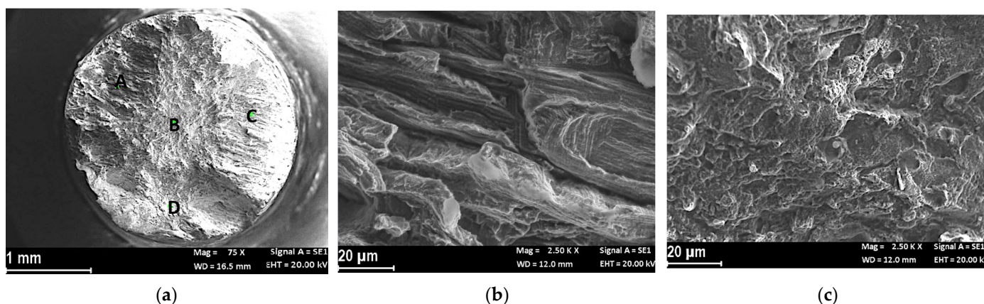
Figure 7. Fractographic analysis of the HT-LPBF specimen after the SSRT test at strain rate 3.15 \times 10^{-6} \text{ s}^{-1} in SOW and cathodic polarization at -1.1 \text{ V} vs. Ag/AgCl: (a) macro image; (b) close-up of the trigger of the fracture (zone A of (a))—zone C has the same morphology of zone A; (c) close-up of the center of the specimen (zone B of (a))—a similar morphology is present in zone D of (a)).
