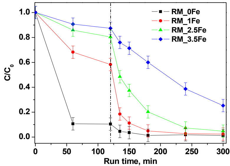
Figure 9. Photocatalytic discoloration of CV aqueous solution with all the studied photocatalysts under visible irradiation (white light).
