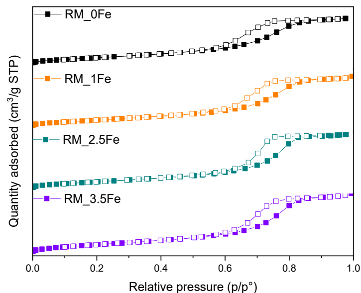
Figure 4. N 2 adsorption/desorption isotherms at -196 °C on the studied samples: RM_0Fe (black squares), RM_1Fe (orange squares), RM_2.5Fe (green squares) and RM_3.5Fe (violet squares). Full and empty symbols refer to adsorption and desorption run, respectively.
