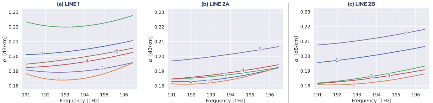
Fig. 6. Physical layer characterization results: retrieved loss coefficient functions for each optical fiber span within the network set in laboratory.
