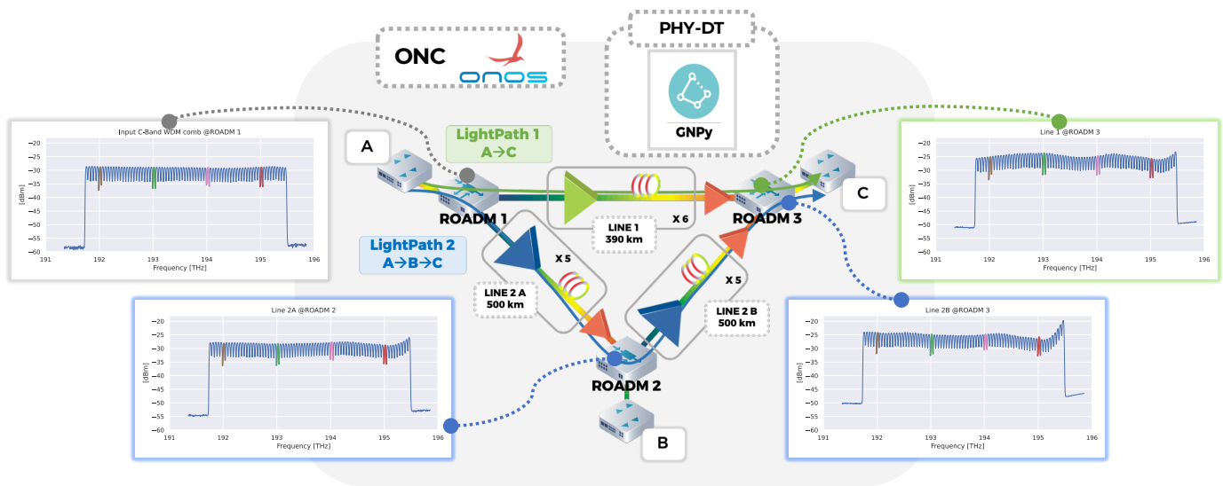
Fig. 4. Experimental setup of the optical network set in laboratory, including the spectra of the C-band WDM comb propagated through the various optical nodes. ONOS holds the role of NOS and GNPy represents the PHY-DT.
