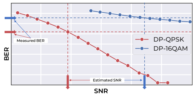
Fig. 5. SNR estimation procedure using TRX B2B curves given the measured BER.
