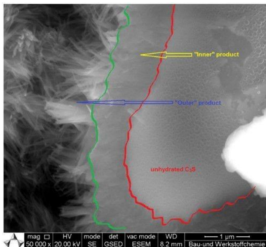
Figure 4. SEM micrograph showing the two types of C-S-H produced during hydration; namely, the “outer” product away from the cement particle surface, occupying the water-filled space and characterized by high porosity, and the “inner” C-S-H formed during later steps of hydration and characterized by low porosity. Reprinted with permission from [77].
