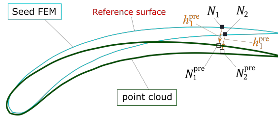
Fig. 5 Pre-morphing step of the improved mesh updating strategy.
