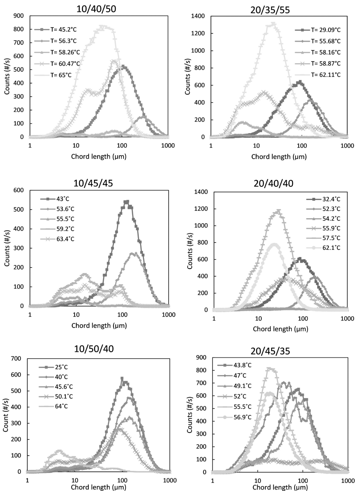
Figure 9. Chord length distributions from laser backscattering for ternary mixtures of Al, acetone, and water (exact w/w concentrations are indicated on top of the figure). Graphs in the same column have same Al amount and increasing concentration of acetone (from top to bottom). Graphs on the same row have the same solvent composition but different Al concentrations.
