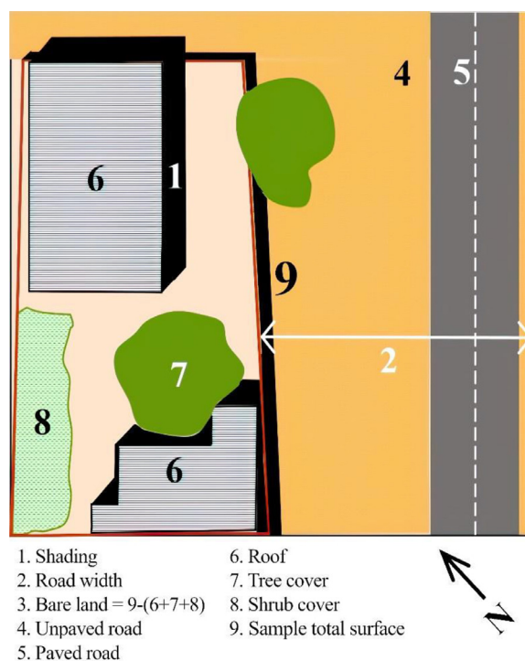
Fig. 9. Landscape metrics.
