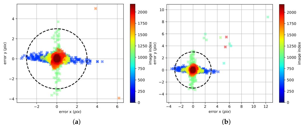
Figure 8. (a) Left cam reprojection error; (b) Right cam reprojection error. ROS kalibr reprojection errors after the calibration optimization process. Mean reprojection error (left cam) px: 0.1627. Mean reprojection error (right cam) px: 0.1734.
