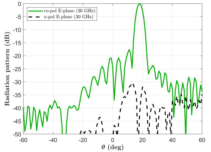
Fig. 5: Computed co-polar and cross-polar components of the radiation pattern in the E-plane, at 30 GHz.
