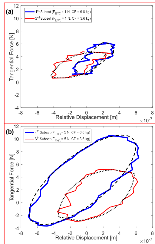
FIGURE 7: HYSTERESIS CYCLES
