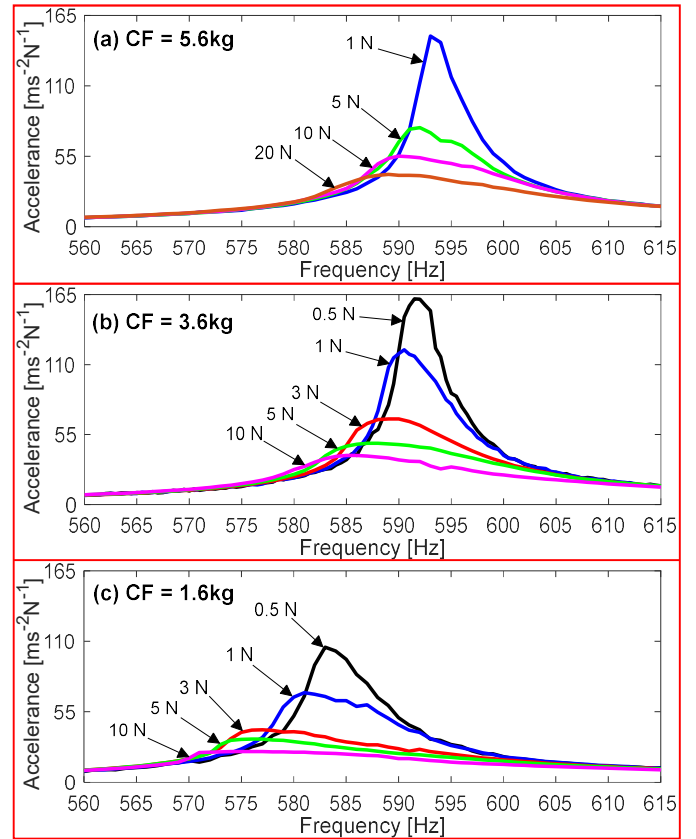
FIGURE 5: NONLINEAR RESPONSE OF THE BLADE WITH AN INCREASING ORDER OF EXCITATION LEVELS
