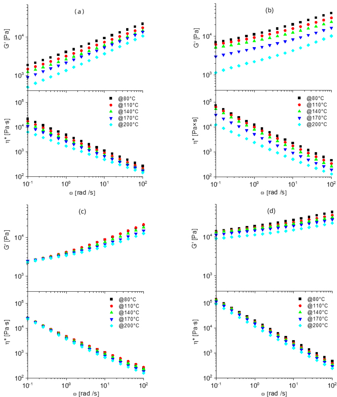
Figure 3. Rheological analyses plots, i.e., storage modulus ( G' ) and complex viscosity ( \eta^* ) for (a) PCL-OH_MDI_1:1_120, (b) PCL-OH_MDI_1:1.33_120, (c) PCL-OH_MDI_1:1_200, and (d) PCL-OH_MDI_1:1.33_200.
