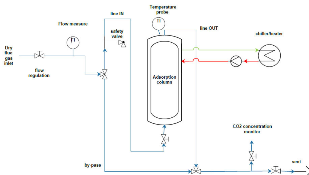
Figure 12. Simplified scheme of a temperature swing process for CO 2 adsorption.
