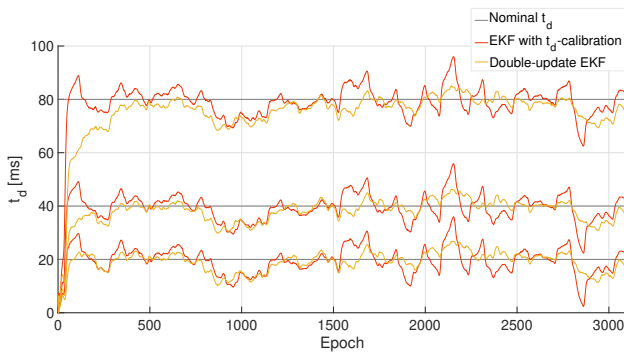
Fig. 7: Time-series of estimated t_d for the simulated trajectory at 20 m/s average receiver speed. Comparison between EKF with naive t_d calibration and double-update EKF. Nominal t_d values of 20 ms, 40 ms and 80 ms are considered.
