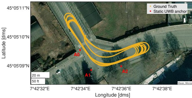
Fig. 12: Map view of the ground reference for the real-world dataset used in the validation of the proposed online time calibration method for GNSS/UWB tight integration.
