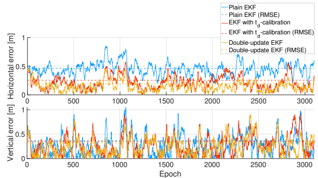
Fig. 8: Horizontal (top) and vertical (bottom) position error trend in ENU-coordinates. Comparison between plain EKF, EKF with naive t_d calibration and double-update EKF. For each architecture, horizontal and vertical RMSE levels are highlighted.
