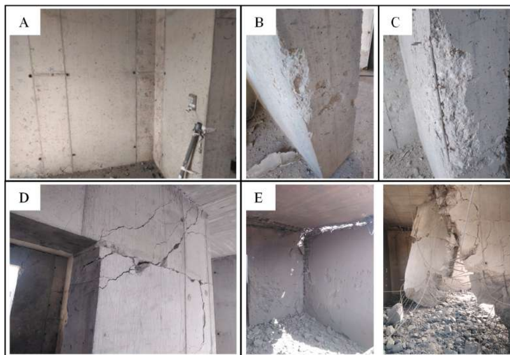
Figure 13. Different effects of IEDs on the interior structure: (A) after the two black powder tests (T1–T2); (B) after the ANFO tests (T3–T4); (C) after the AN/AL tests (T5–T6); (D) after the first PG2 test (T7); (E) after the second PG2 test (T8).
