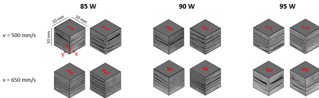
Fig. 4. Visual reconstruction of all faces of the samples produced with process parameters indicated by the SST software.
