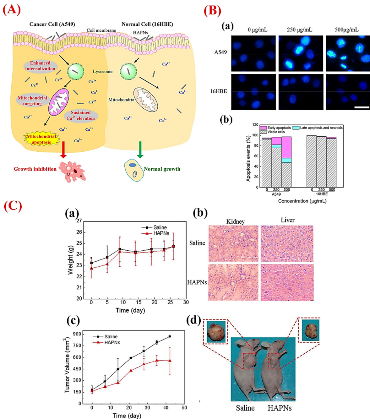
Figure 3. (A) HAP NPs can induce cytotoxicity in cancer cells (adenocarcinoma human alveolar basal epithelial cells, A549 cells) through mitochondria-mediated apoptosis due to higher internalization as compared to normal cells (human bronchial epidermal cells, 16HBE cells). (B) Fluorescent micrographs of cells (a) before and after treatment with different doses of HAp NPs for 48 h (scale bar: 20 µm) and (b) Annexin V-FITC/PI double staining analysis of the cells showing apoptosis ratios in A549 and 16HBE cells post-treatment with HAp NPs. (C) In vivo tumor inhibition efficacy of HAP NPs: the effect of the HAP NPs treatments on changes in the body weight of healthy nude mice at a dosage of 40 mg/kg (three times a week) (a); histology evaluation (hematoxylin and eosin staining) of kidney and liver samples from healthy nude mice treated with saline or HAP NPs (40 mg/kg) on day 26 (magnification 200×) (b); tumor growth curves of nude mice bearing xenografted A549 cells treated with 40 mg/kg of HAP NPs three times a week (c); and macroscopic images of mice and excised tumors from saline or HAP NPs-treated groups at the time of sacrifice (d). Reproduced with permission from ref. [98].
