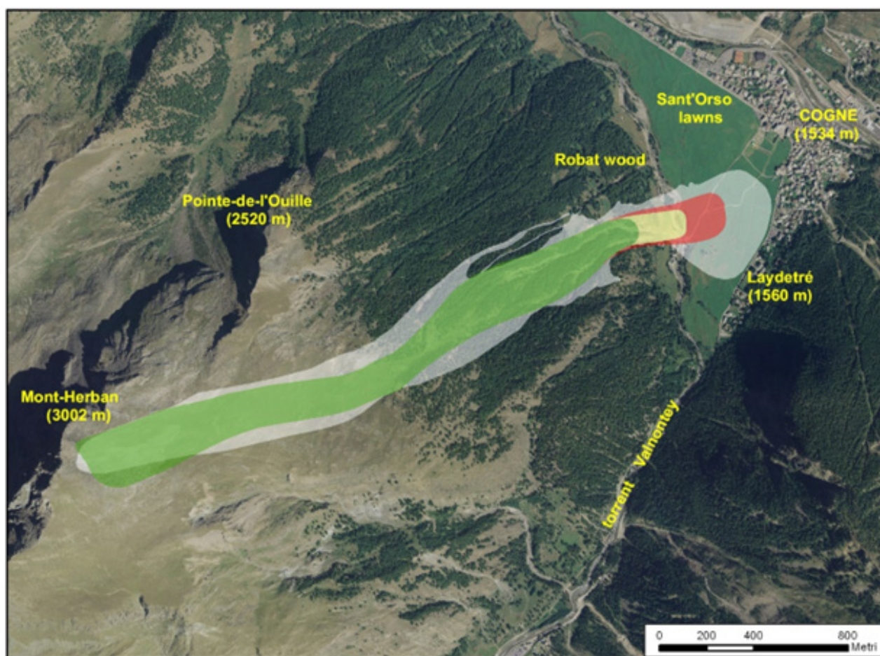
Figure 1: The avalanche hazard map (Carta Ambiti inedificabili Art. 37 LR 11/98) of the n. 52 – Buthier avalanche basin in Cogné – AO (IT) with the three avalanche danger degrees (high in red, medium in yellow and low in green) based on a range of avalanche impact pressure (respectively higher than 3t/mq, between 0,5 and 3t/mq and less than 0,5t/mq). In white the perimeter of the avalanche event of December 15th, 2008.
